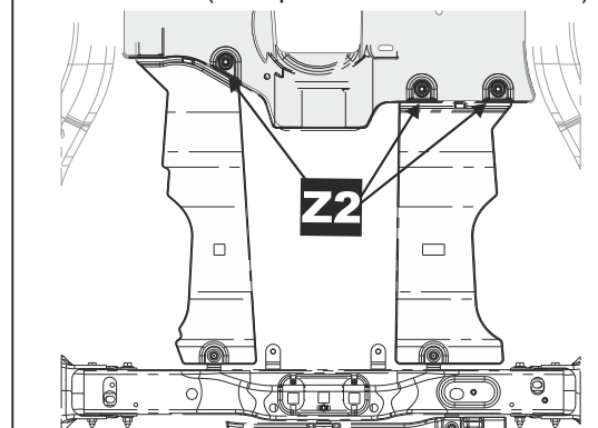
VJA300L-(except VJA300L-GMUZZW)
