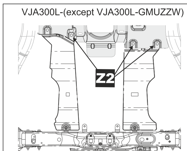
FJA300L-(except FJA300L-GMUZYW)
